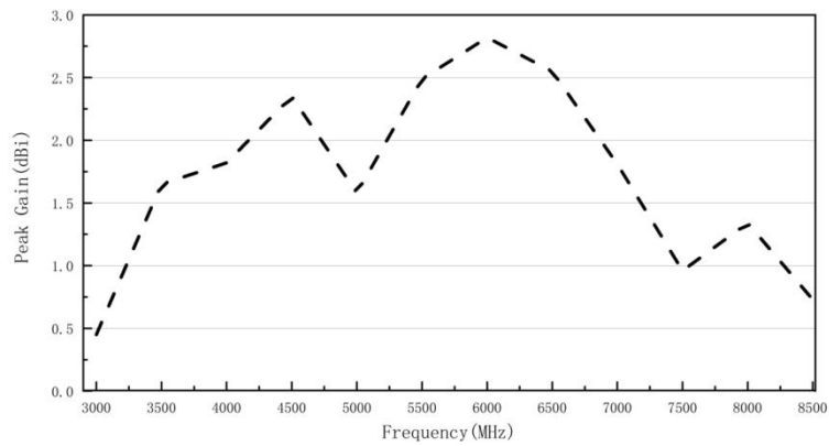
Figure 8. MAN3080C86 Peak Gain
