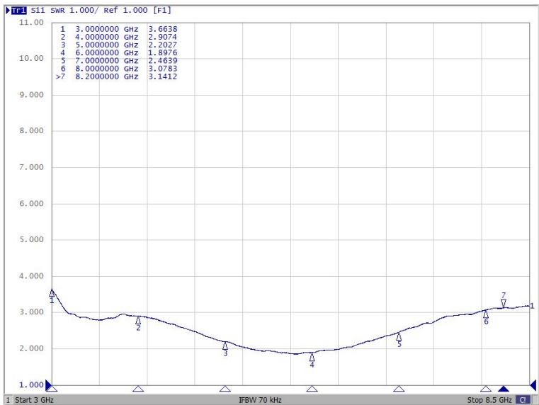
Figure 5. MAN3080C86 VSWR
