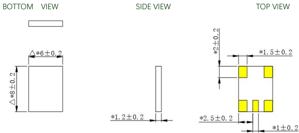
Figure 1. MAN3080C86 View (Unit: mm)
