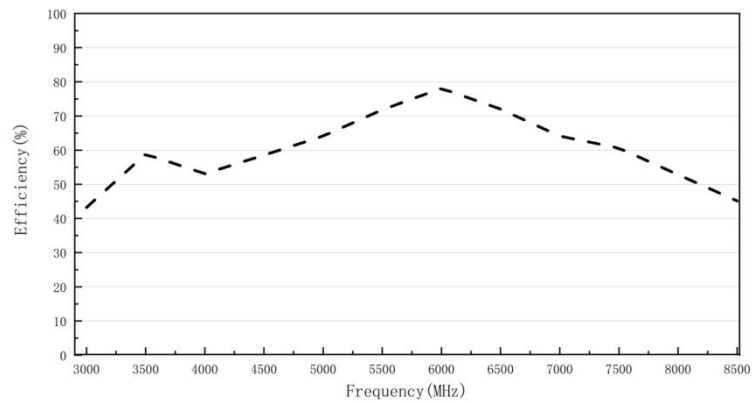
Figure 7. MAN3080C86 Total Efficiency
