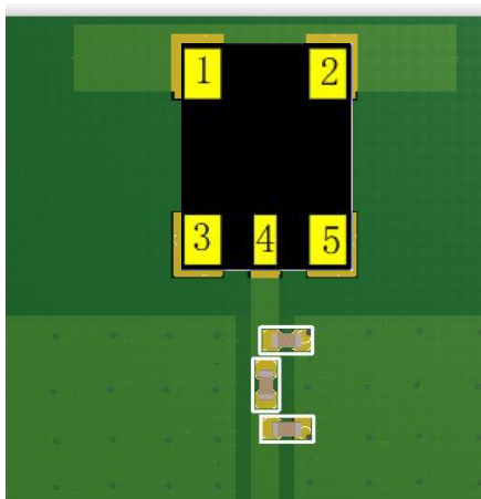
Figure 4. MAN3080C86 Matching Circuit (Unit: mm)
