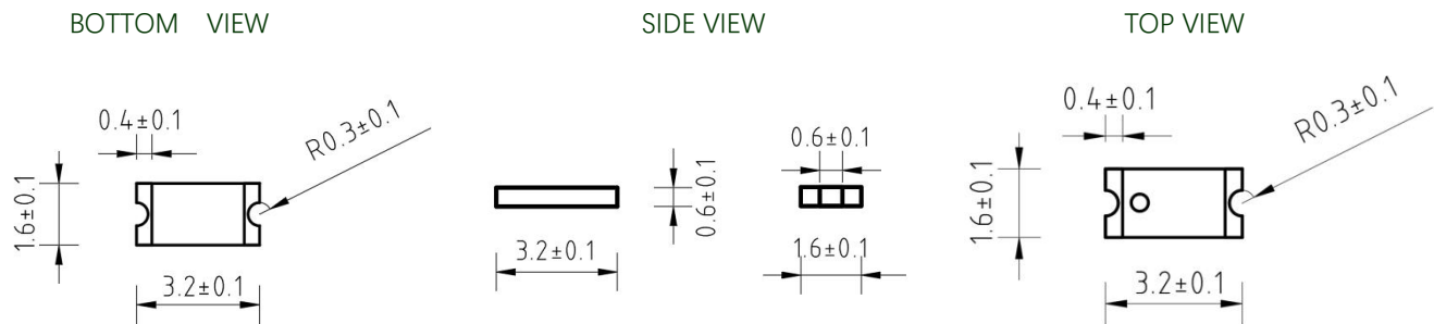
Figure 1. MAN2450C32 View (Unit: mm)
