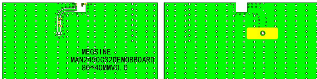
Figure 2. MAN2450C32 PCB Layout (Unit: mm)
