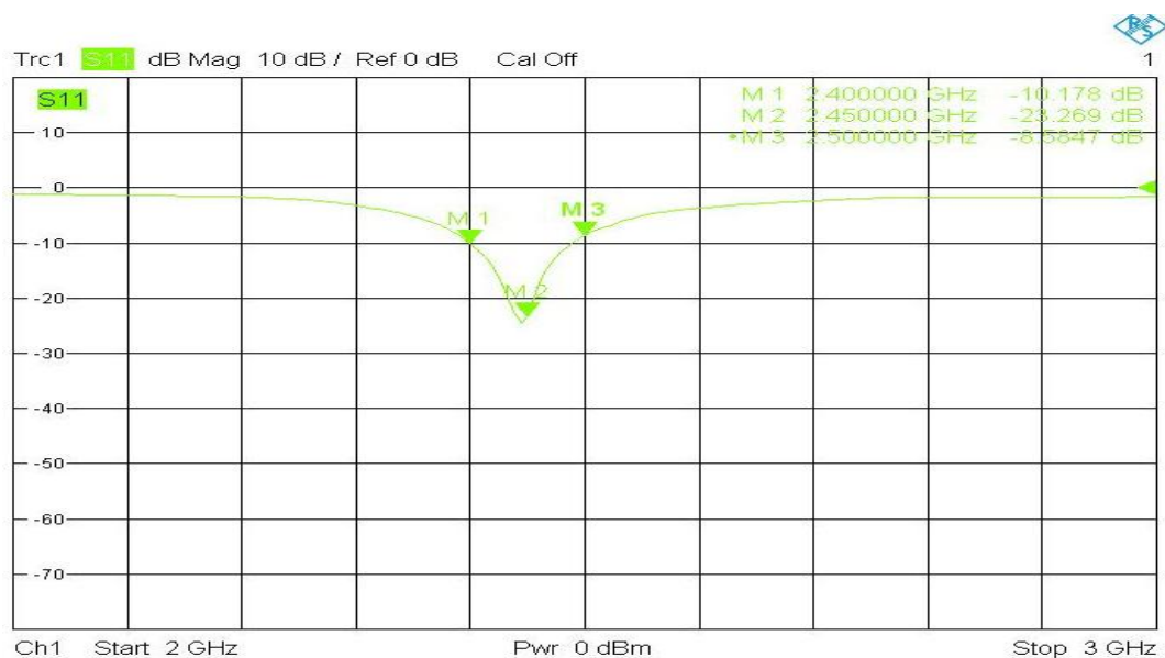
Figure 6. MAN2450C32 Return Loss
