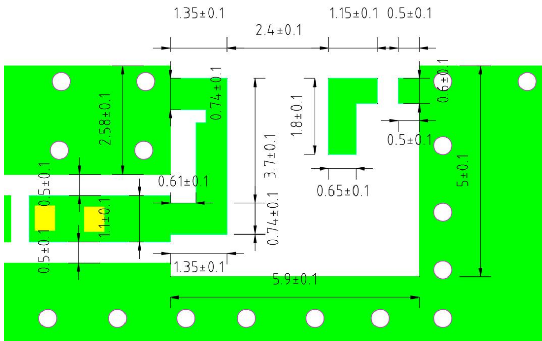
Figure 3. MAN2450C32 Antenna Layout (Unit: mm)
