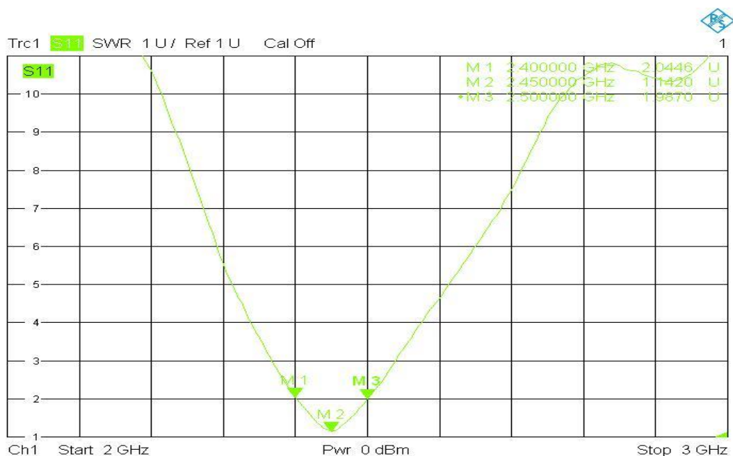
Figure 5. MAN2450C32 VSWR
