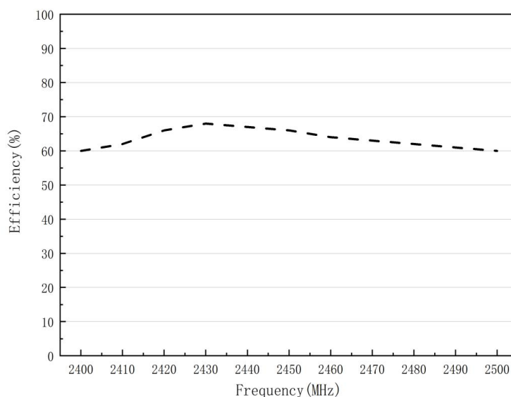
Figure 8. MAN2450C32 Total Efficiency
