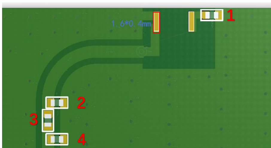
Figure 4. MAN2450C32 Foot Print (Unit: mm)
