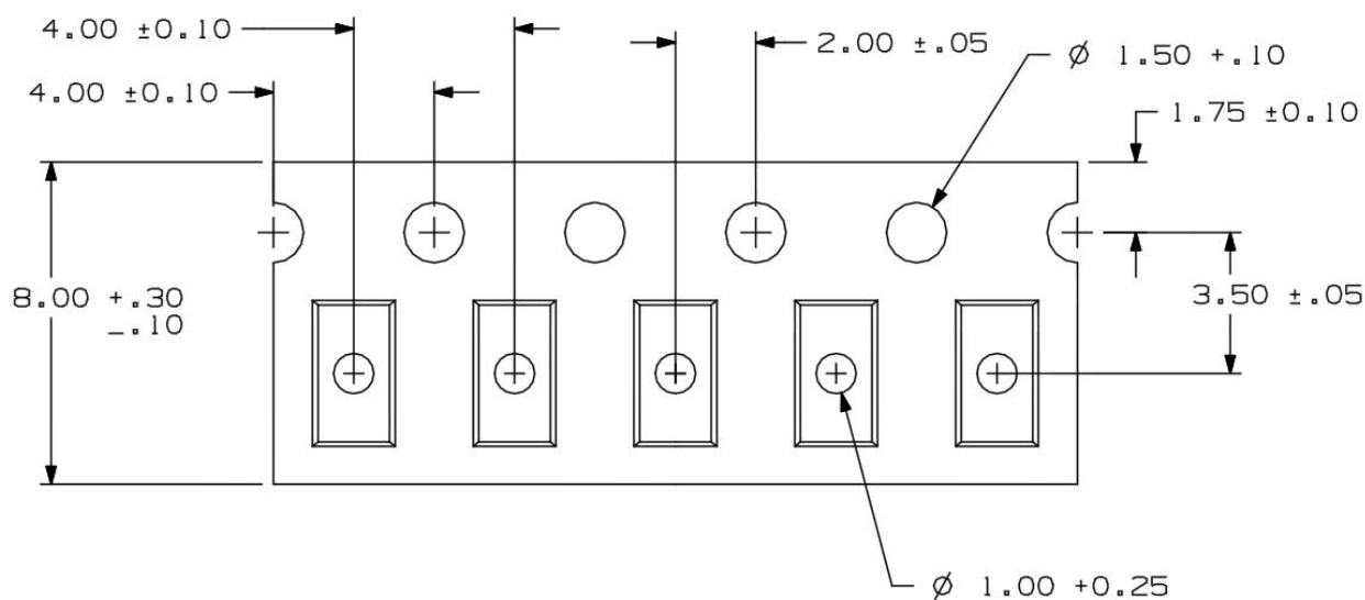
Figure 11. Packaging Information
