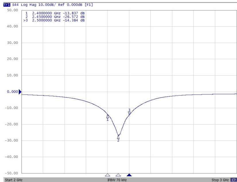
Figure 6. MAN2450L42 Return Loss
