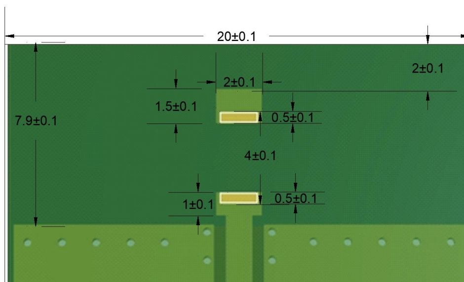
Figure 3. MAN2450L42 Antenna Layout (Unit: mm)
