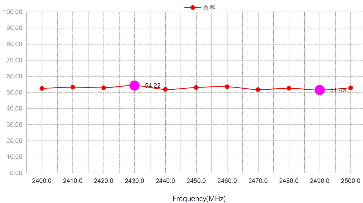
Figure 8. MAN2450L42 Total Efficiency
