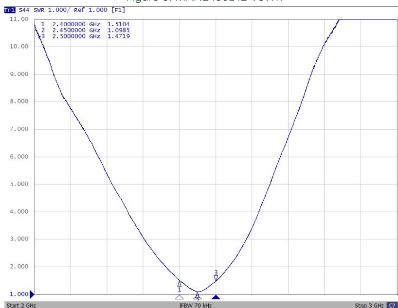
Figure 5. MAN2450L42 VSWR
