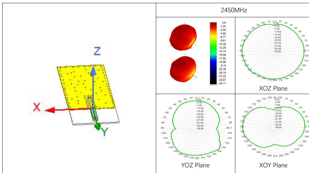
Figure 10. Radiation Pattern
