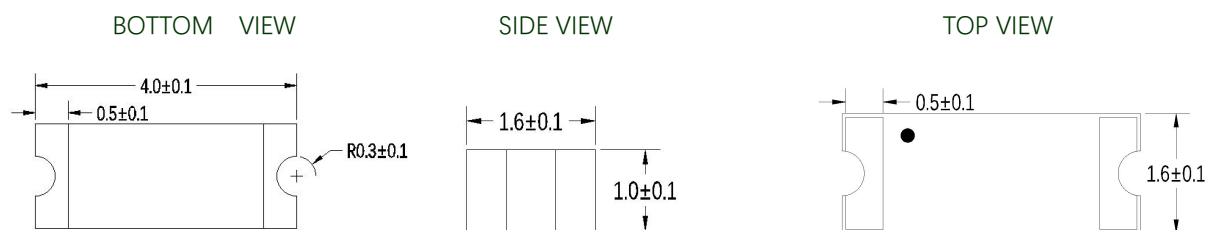
Figure 1. MAN2450L42 View (Unit: mm)
